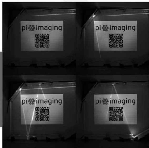
Track short burst of light scattering in water, traveling at 225 million m/s and imaged with 17 ps time resolution.
